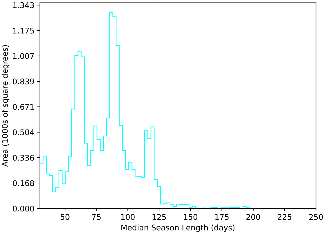
too_elab_heavy_r32_d3_gz_v3.4_10yrs WFD u band: Median Season Length
