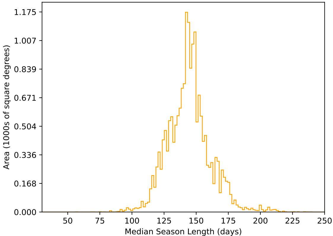
too_elab_heavy_r32_d3_gz_v3.4_10yrs WFD r band: Median Season Length
