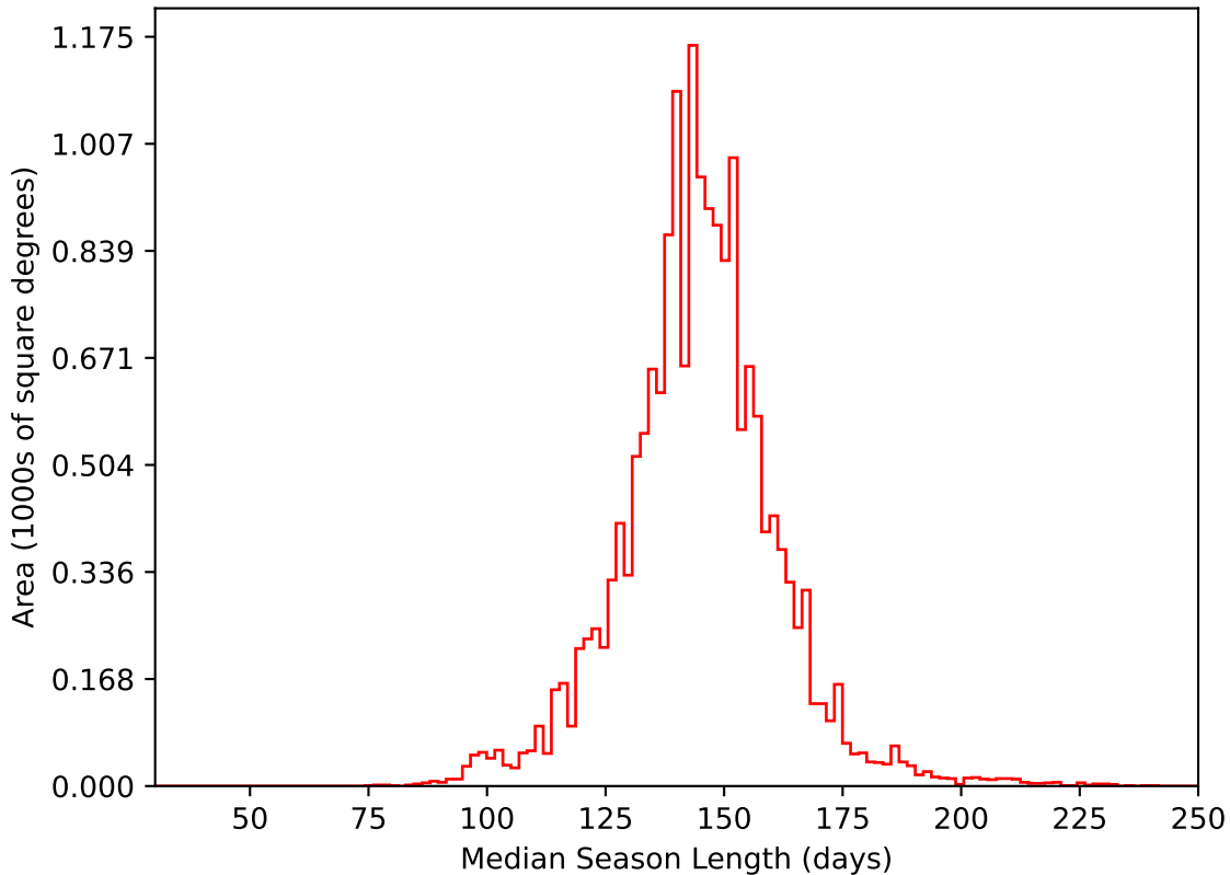
too_elab_heavy_r32_d3_gz_v3.4_10yrs WFD i band: Median Season Length
