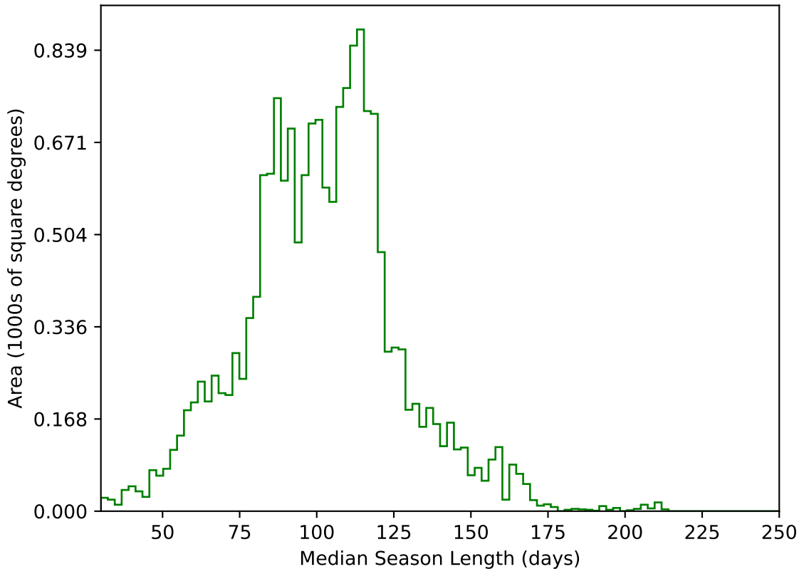
too_elab_heavy_r32_d3_gz_v3.4_10yrs WFD g band: Median Season Length
