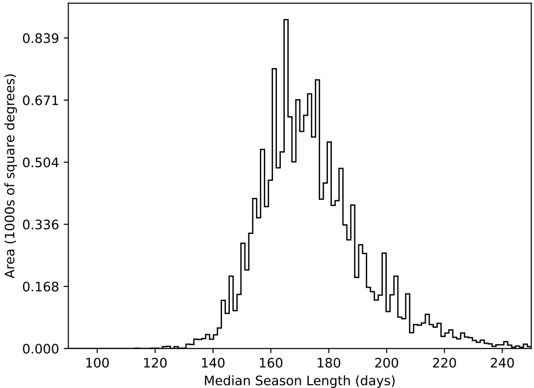
too_elab_heavy_r32_d3_gz_v3.4_10yrs WFD all bands: Median Season Length
