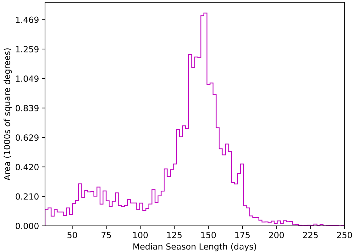
too_elab_heavy_r32_d3_gz_v3.4_10yrs All sky z band: Median Season Length
