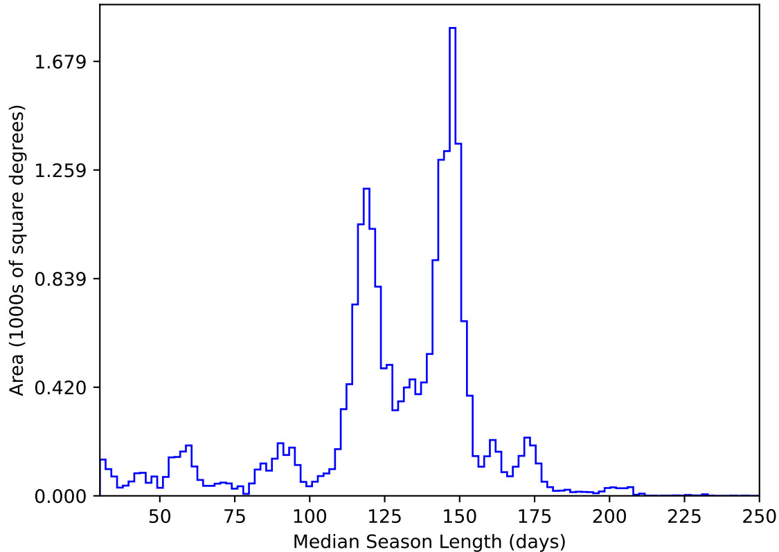
too_elab_heavy_r32_d3_gz_v3.4_10yrs All sky y band: Median Season Length
