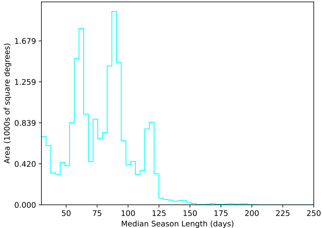
too_elab_heavy_r32_d3_gz_v3.4_10yrs All sky u band: Median Season Length
