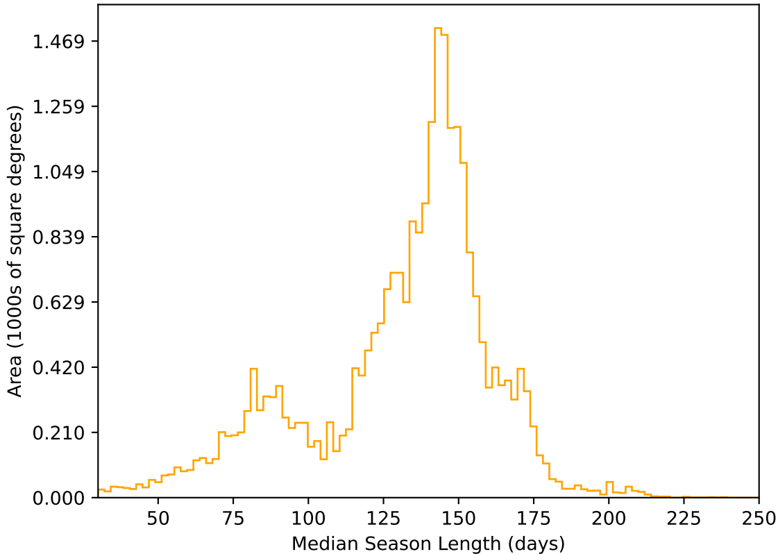
too_elab_heavy_r32_d3_gz_v3.4_10yrs All sky r band: Median Season Length
