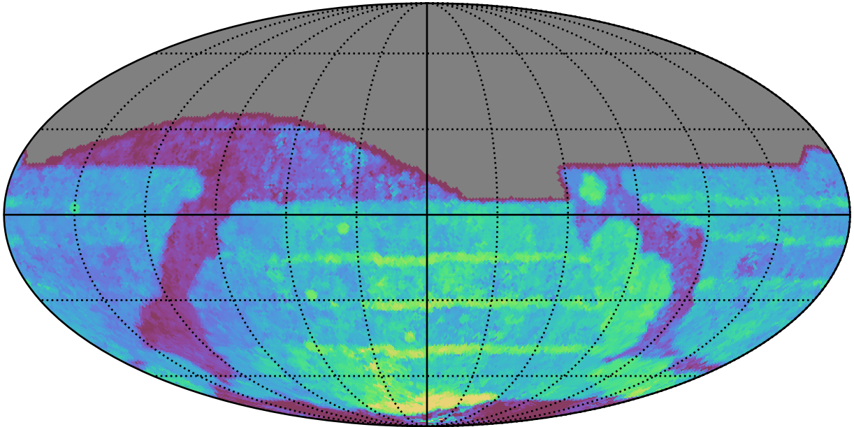
too_elab_heavy_r32_d3_gz_v3.4_10yrs All sky all bands: Median Season Length
