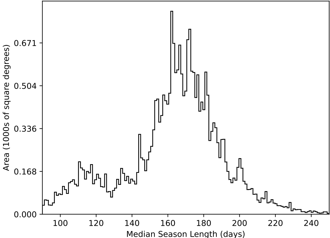
too_elab_heavy_r32_d3_gz_v3.4_10yrs All sky all bands: Median Season Length
