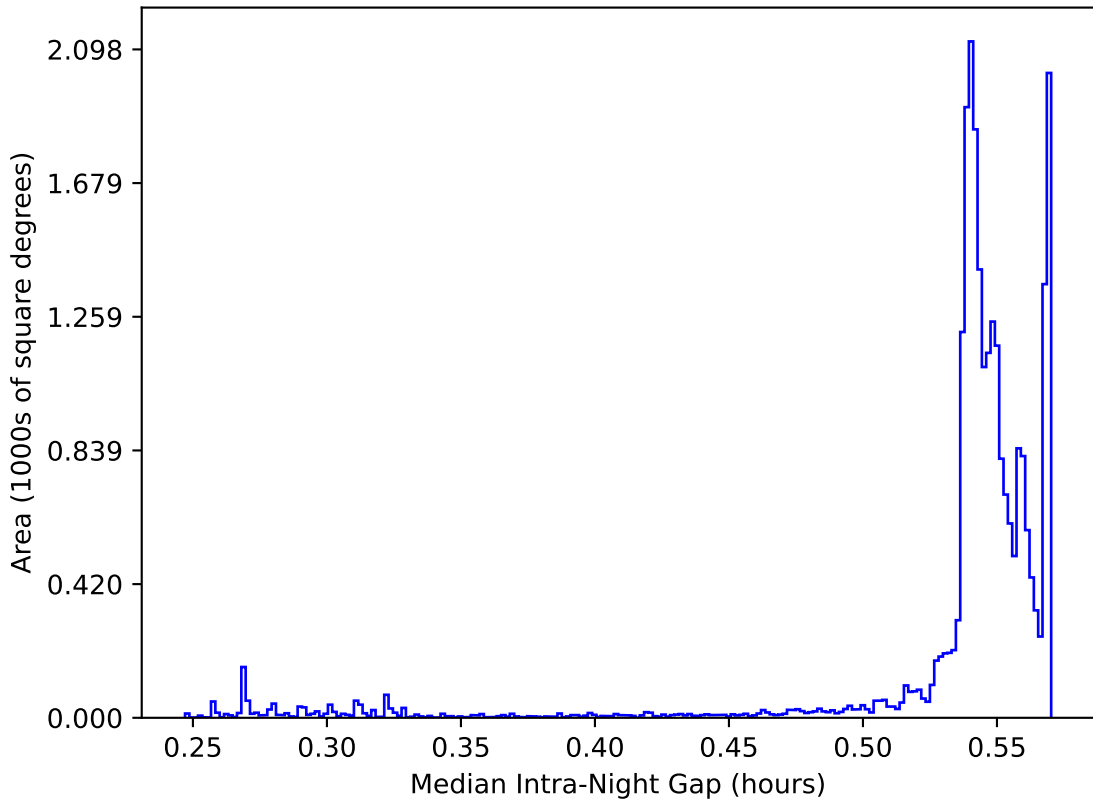
too_elab_heavy_r32_d3_gz_v3.4_10yrs All sky: Median Intra-Night Gap
