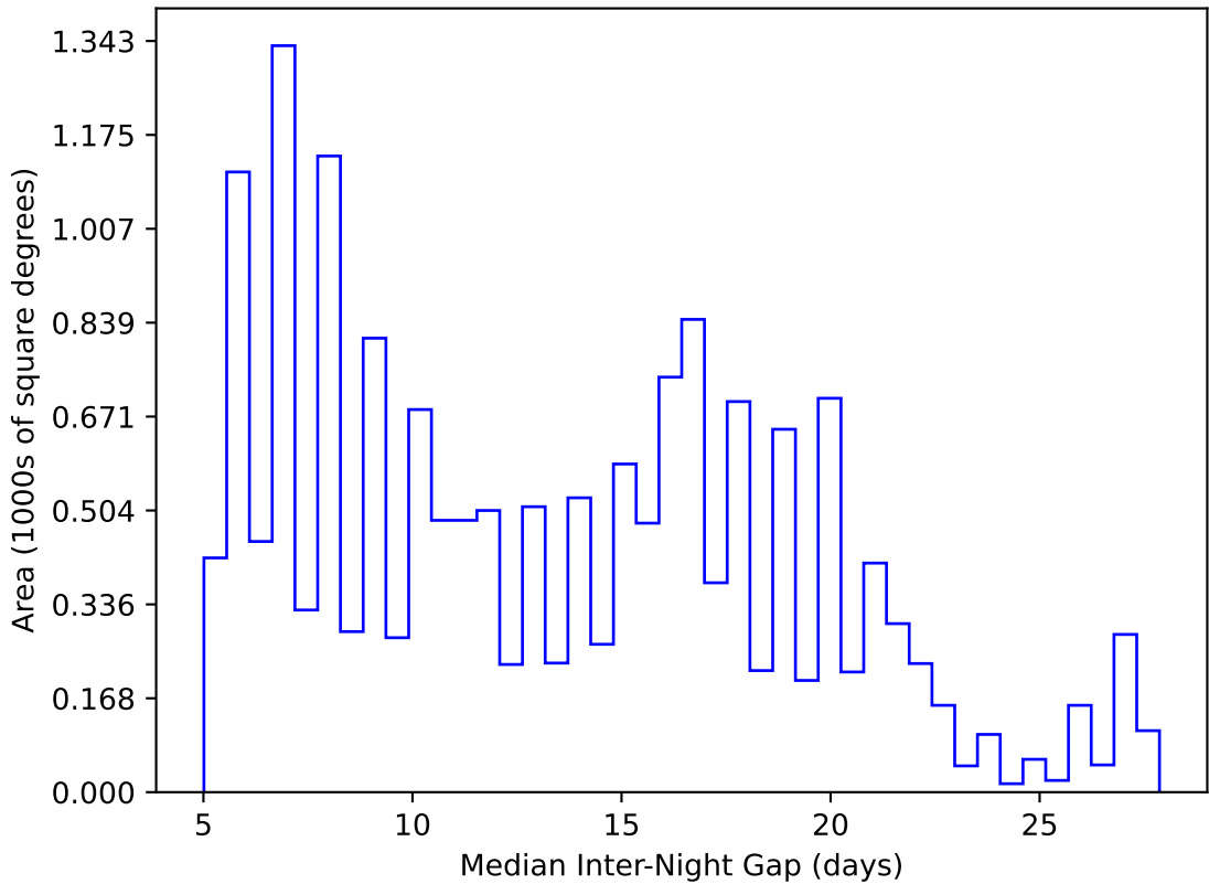
too_elab_heavy_r32_d3_gz_v3.4_10yrs WFD y band: Median Inter-Night Gap
