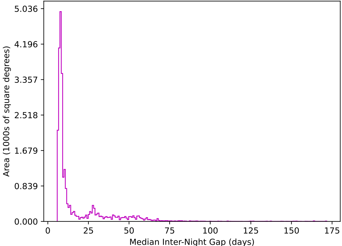
too_elab_heavy_r32_d3_gz_v3.4_10yrs All sky z band: Median Inter-Night Gap
