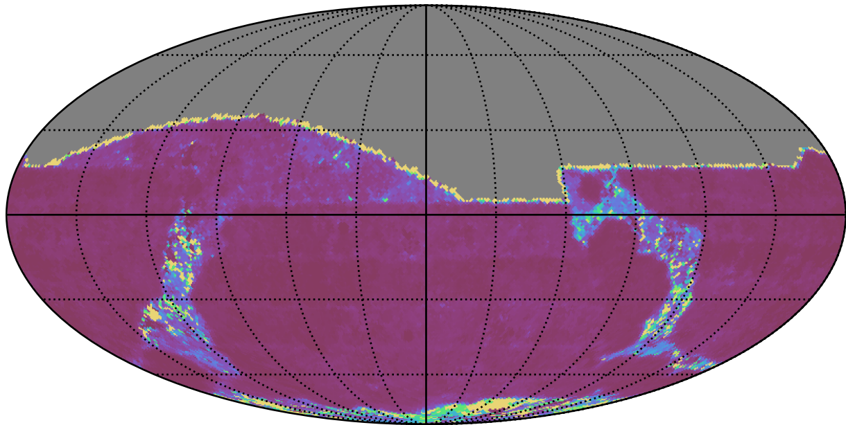
too_elab_heavy_r32_d3_gz_v3.4_10yrs All sky g band: Median Inter-Night Gap
