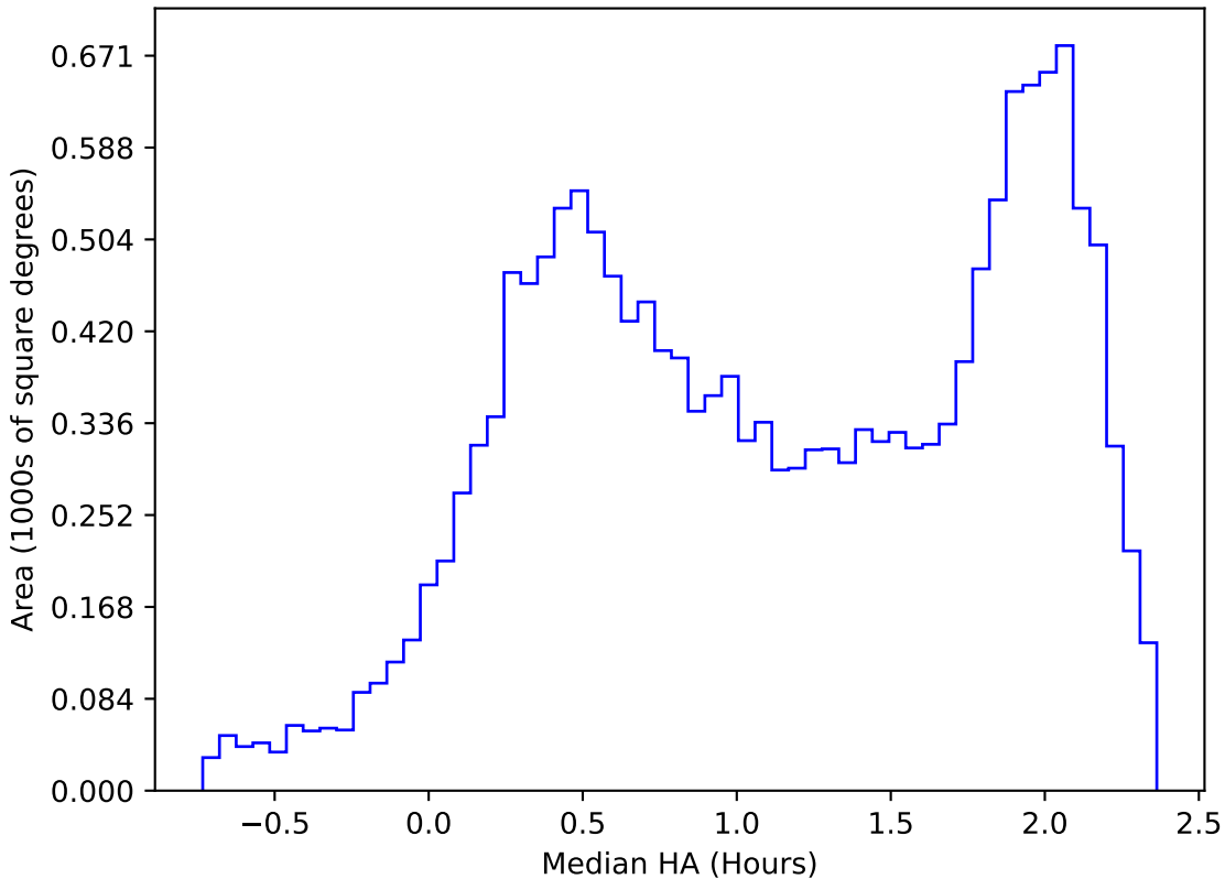
too_elab_heavy_r32_d3_gz_v3.4_10yrs WFD z band: Median HA
