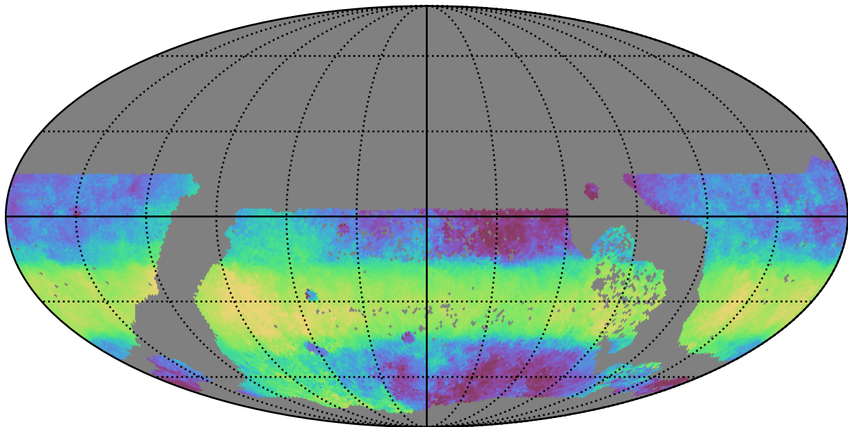
too_elab_heavy_r32_d3_gz_v3.4_10yrs WFD y band: Median HA
