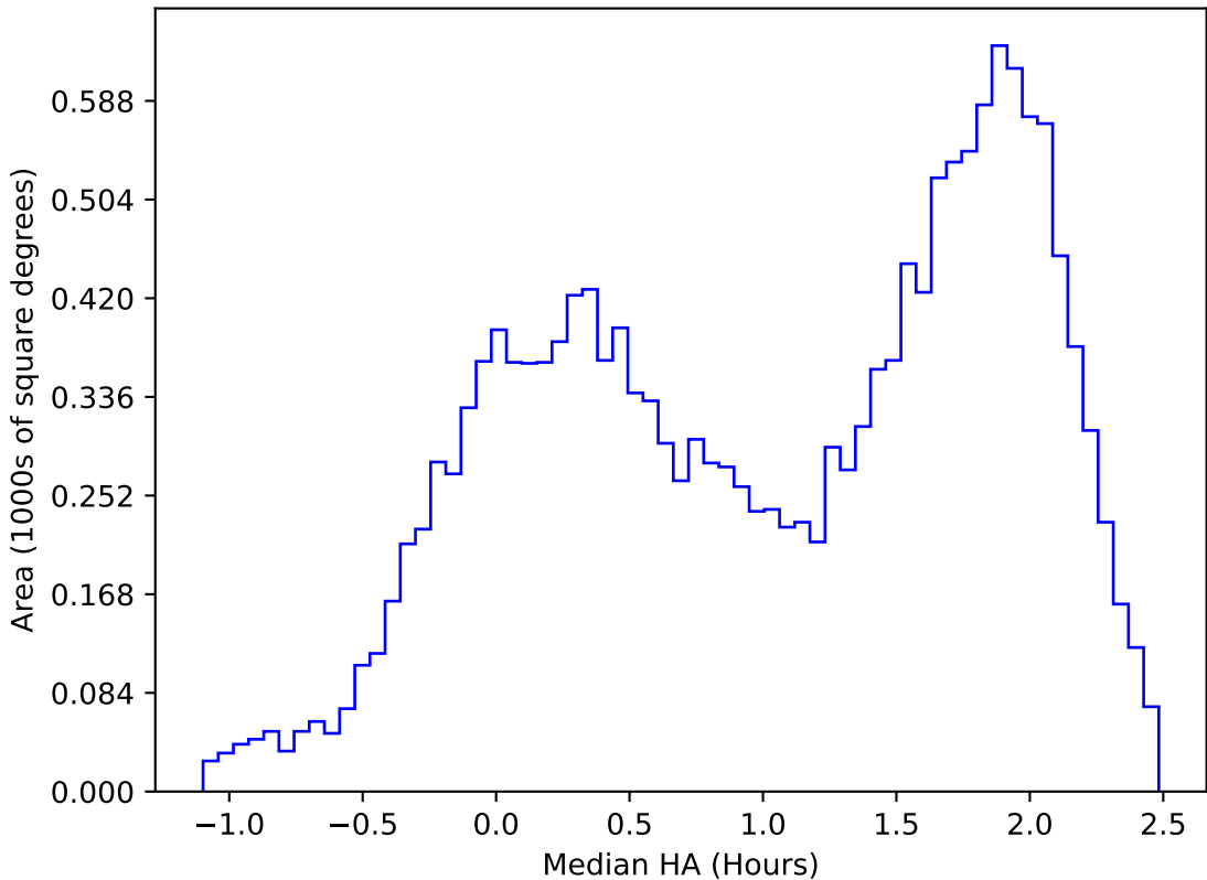
too_elab_heavy_r32_d3_gz_v3.4_10yrs WFD u band: Median HA
