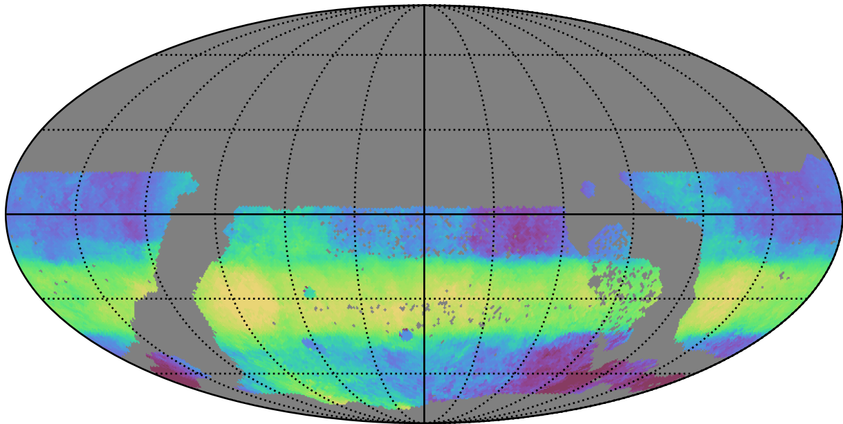
too_elab_heavy_r32_d3_gz_v3.4_10yrs WFD r band: Median HA
