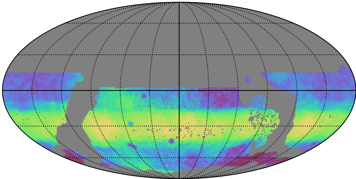
too_elab_heavy_r32_d3_gz_v3.4_10yrs WFD i band: Median HA
