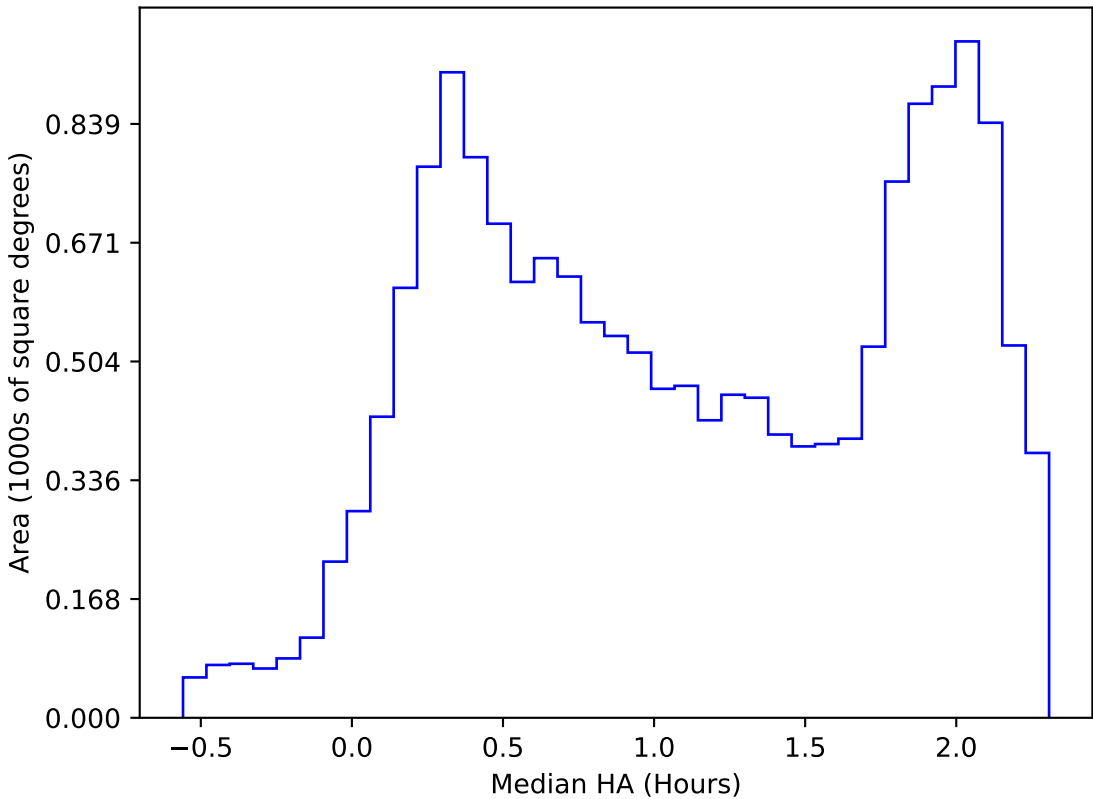
too_elab_heavy_r32_d3_gz_v3.4_10yrs WFD i band: Median HA
