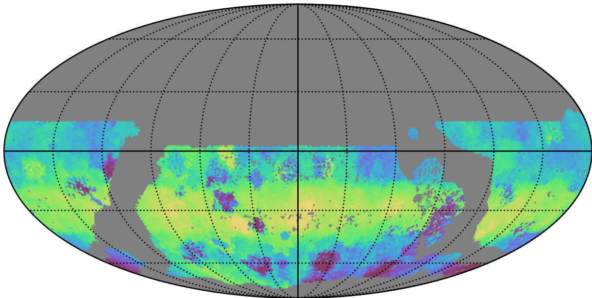
too_elab_heavy_r32_d3_gz_v3.4_10yrs WFD g band: Median HA
