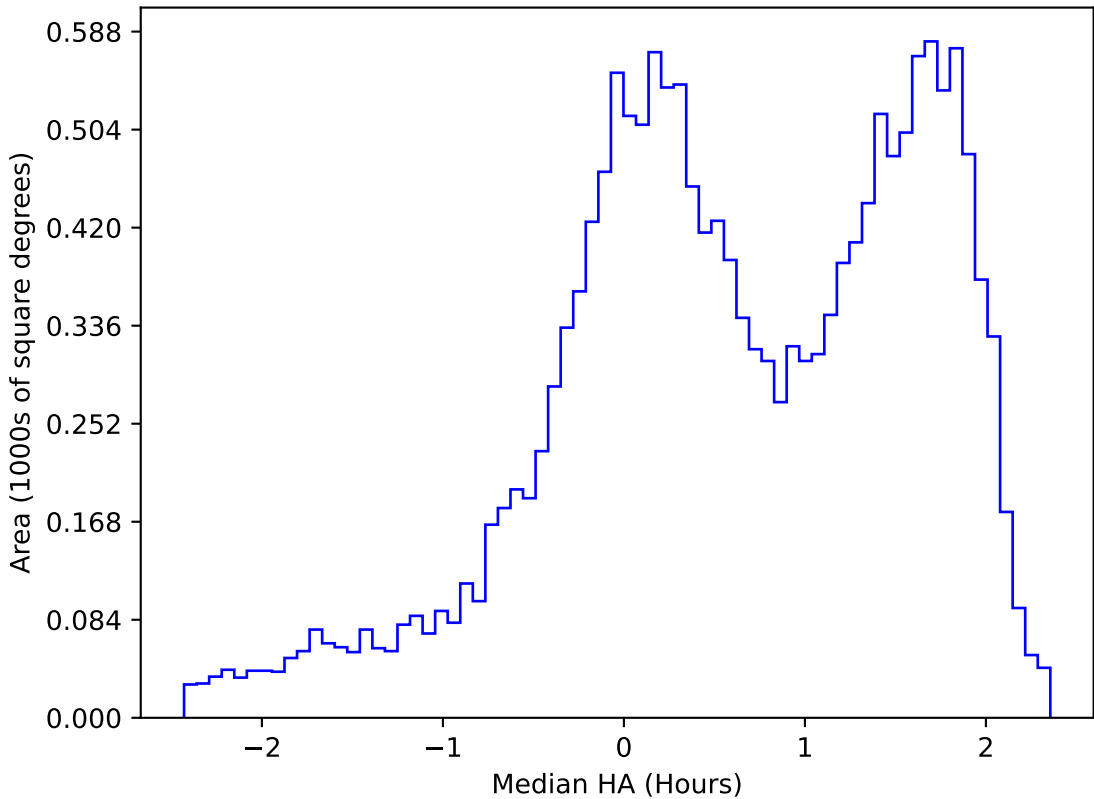
too_elab_heavy_r32_d3_gz_v3.4_10yrs WFD g band: Median HA
