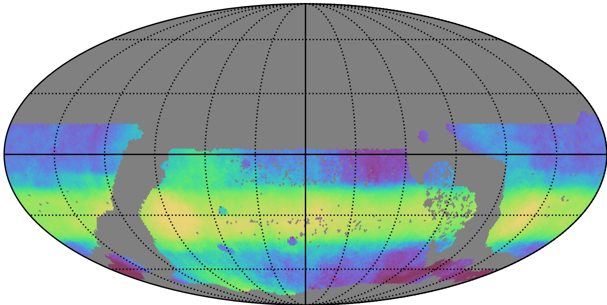
too_elab_heavy_r32_d3_gz_v3.4_10yrs WFD all bands: Median HA
