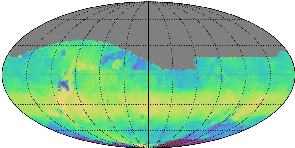
too_elab_heavy_r32_d3_gz_v3.4_10yrs All sky z band: Median HA
