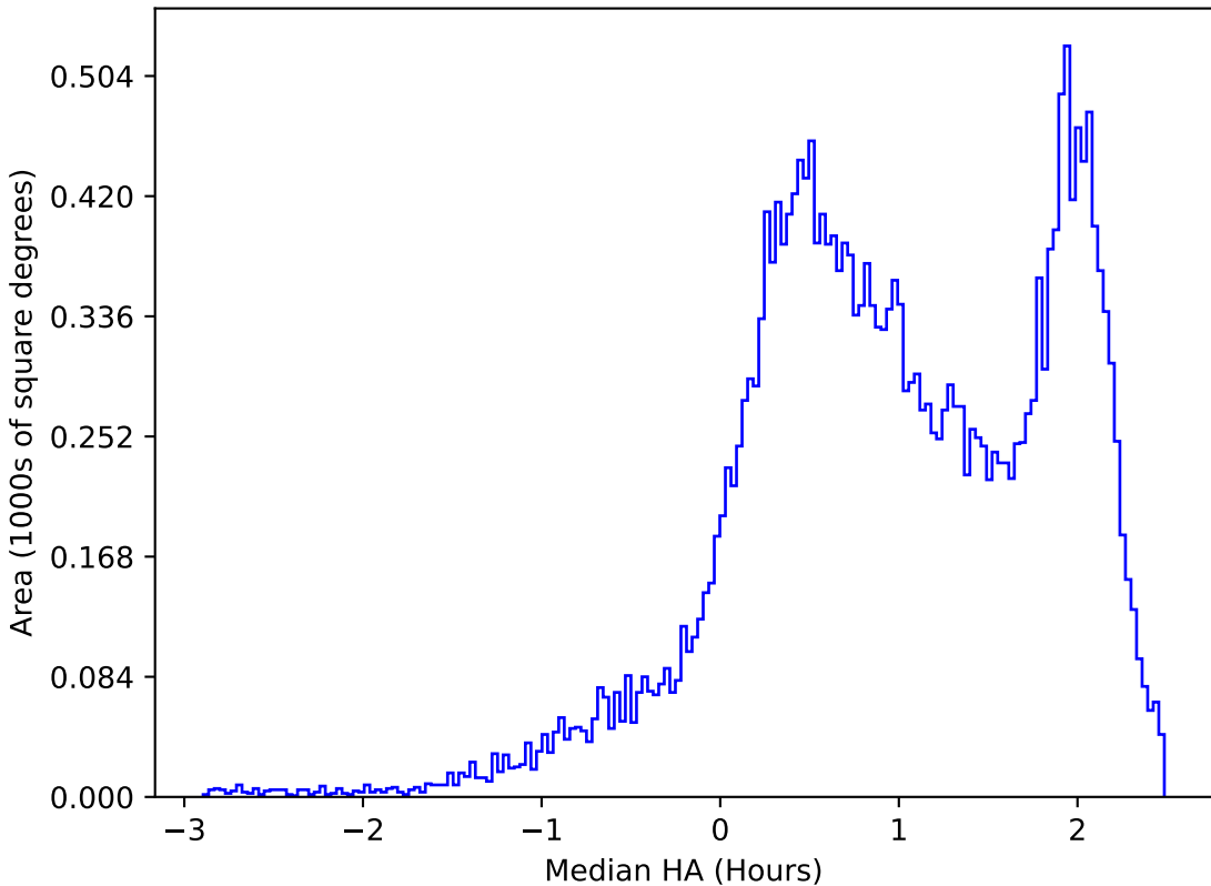
too_elab_heavy_r32_d3_gz_v3.4_10yrs All sky z band: Median HA
