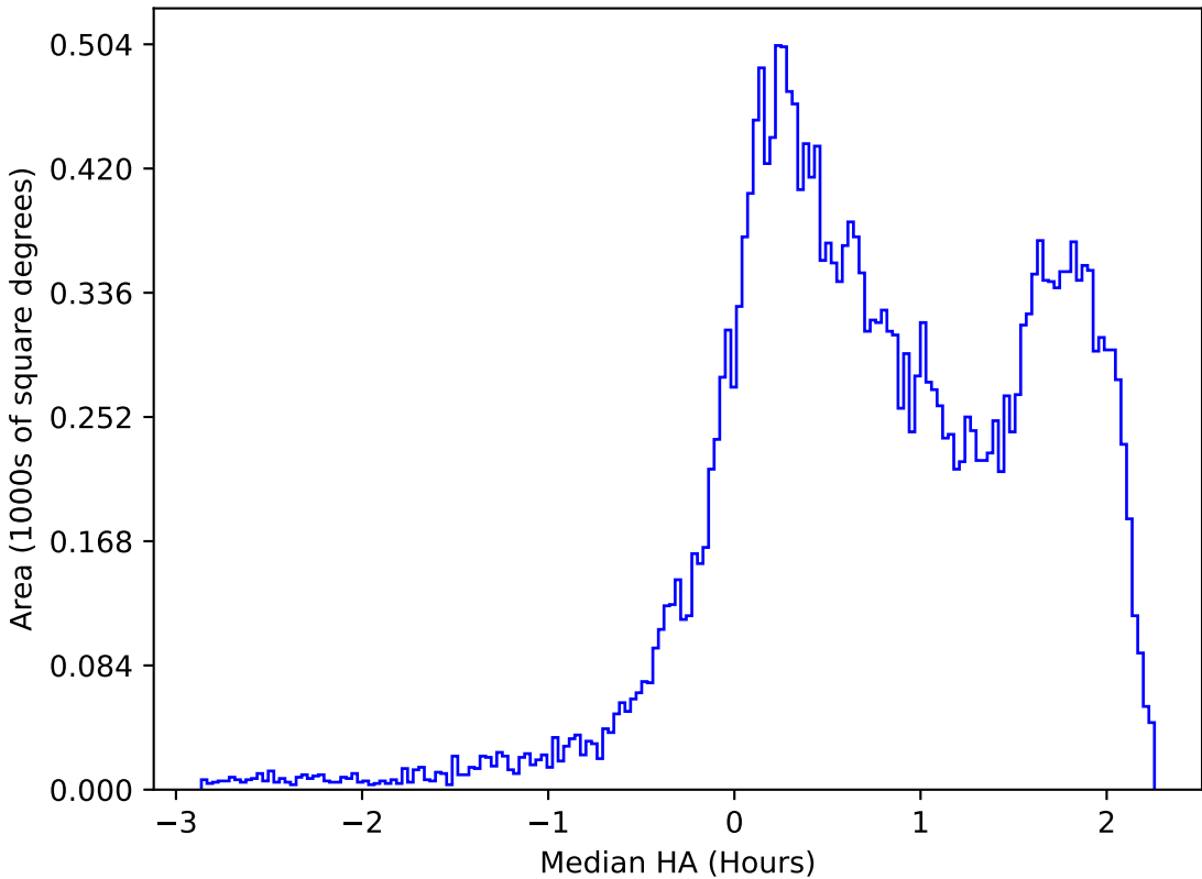
too_elab_heavy_r32_d3_gz_v3.4_10yrs All sky r band: Median HA
