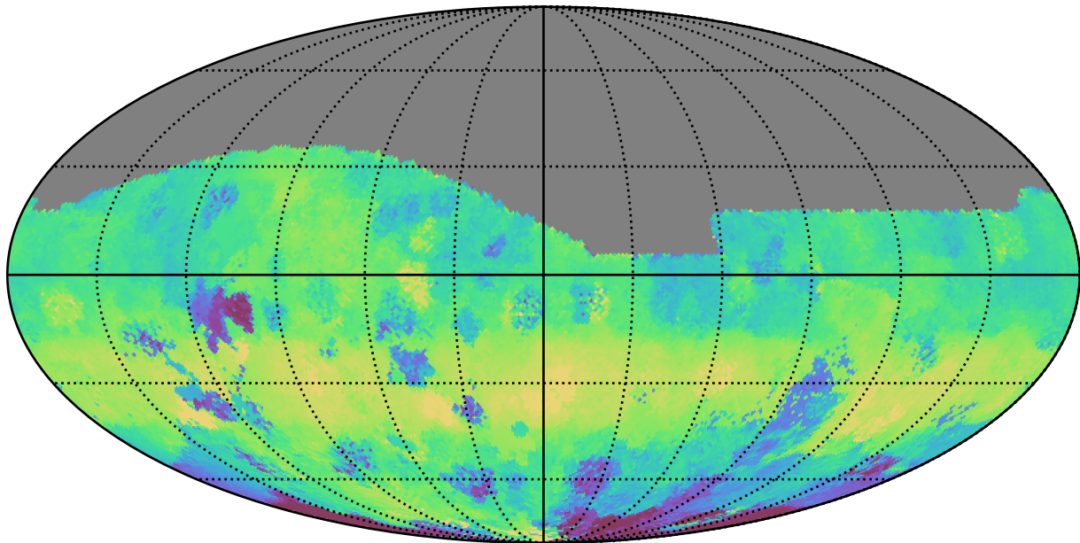
too_elab_heavy_r32_d3_gz_v3.4_10yrs All sky g band: Median HA
