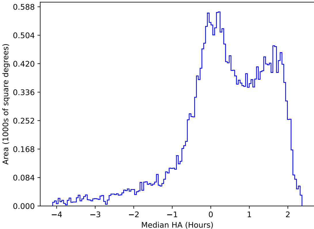
too_elab_heavy_r32_d3_gz_v3.4_10yrs All sky g band: Median HA
