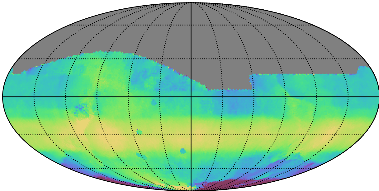
too_elab_heavy_r32_d3_gz_v3.4_10yrs All sky all bands: Median HA
