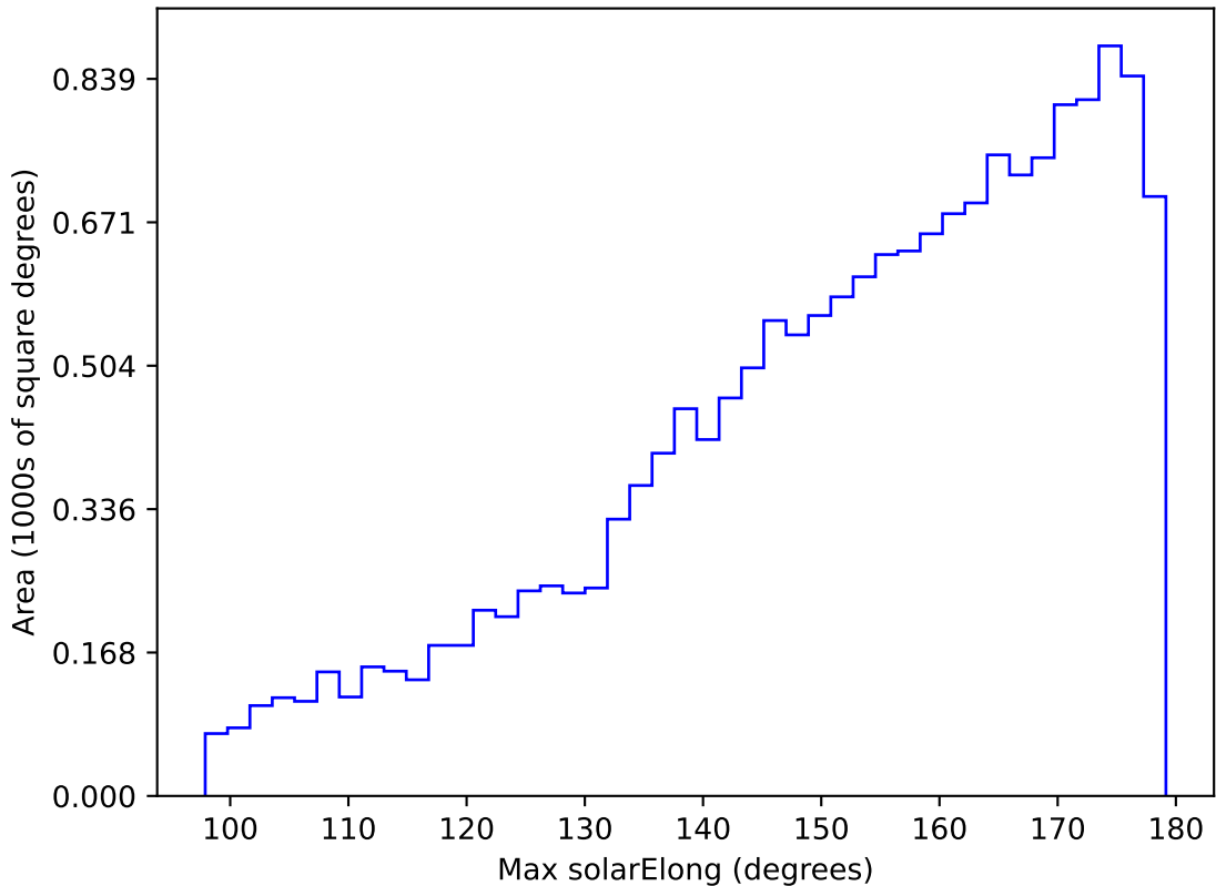
too_elab_heavy_r32_d3_gz_v3.4_10yrs WFD u band: Max solarElong
