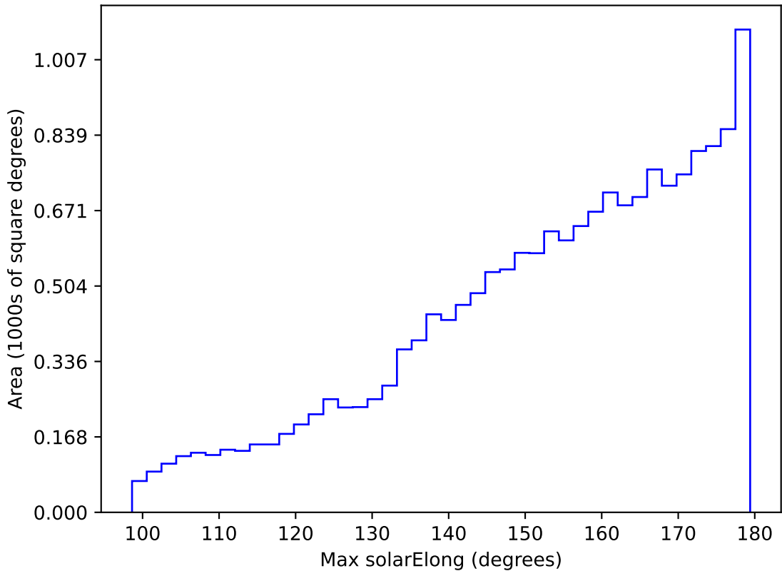
too_elab_heavy_r32_d3_gz_v3.4_10yrs WFD r band: Max solarElong
