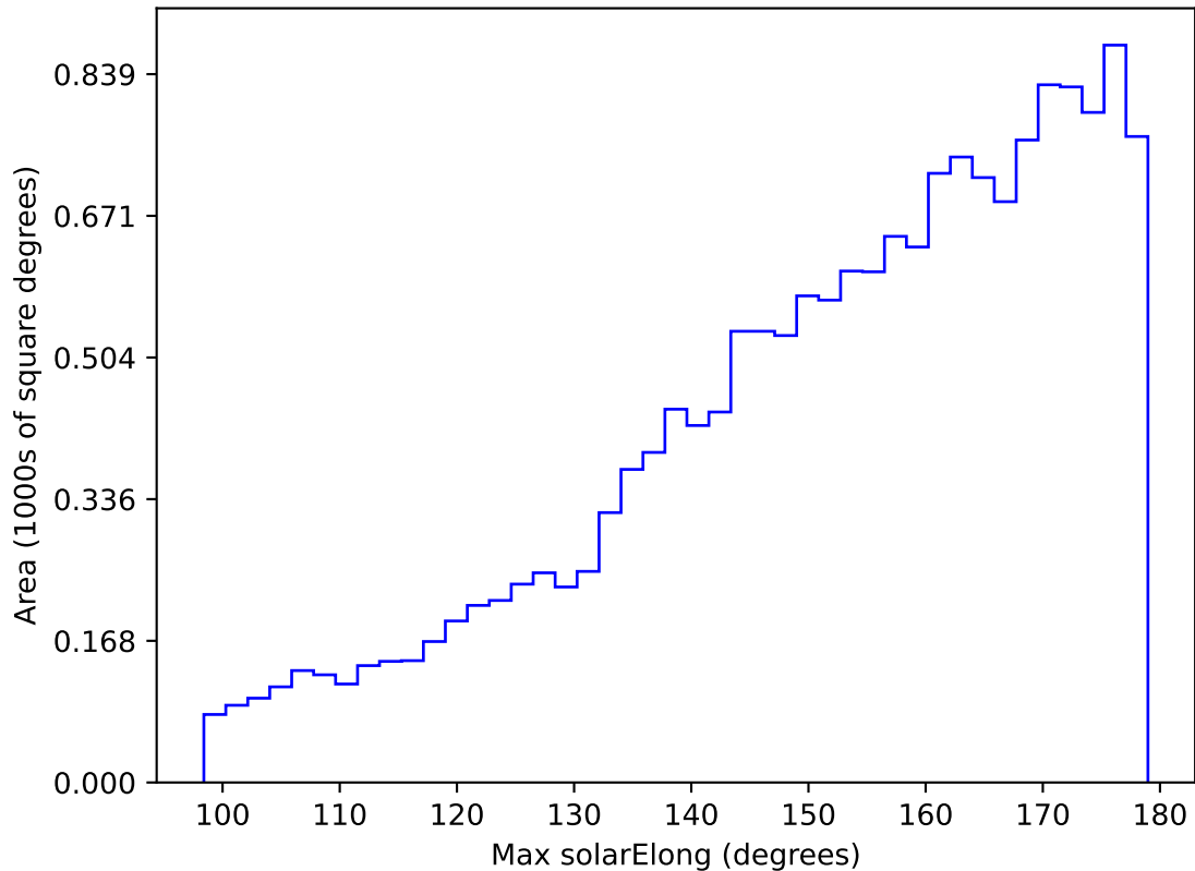
too_elab_heavy_r32_d3_gz_v3.4_10yrs WFD g band: Max solarElong
