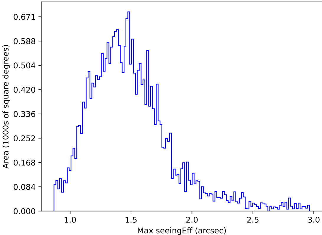
too_elab_heavy_r32_d3_gz_v3.4_10yrs Yr 1 z band: Max seeingEff
