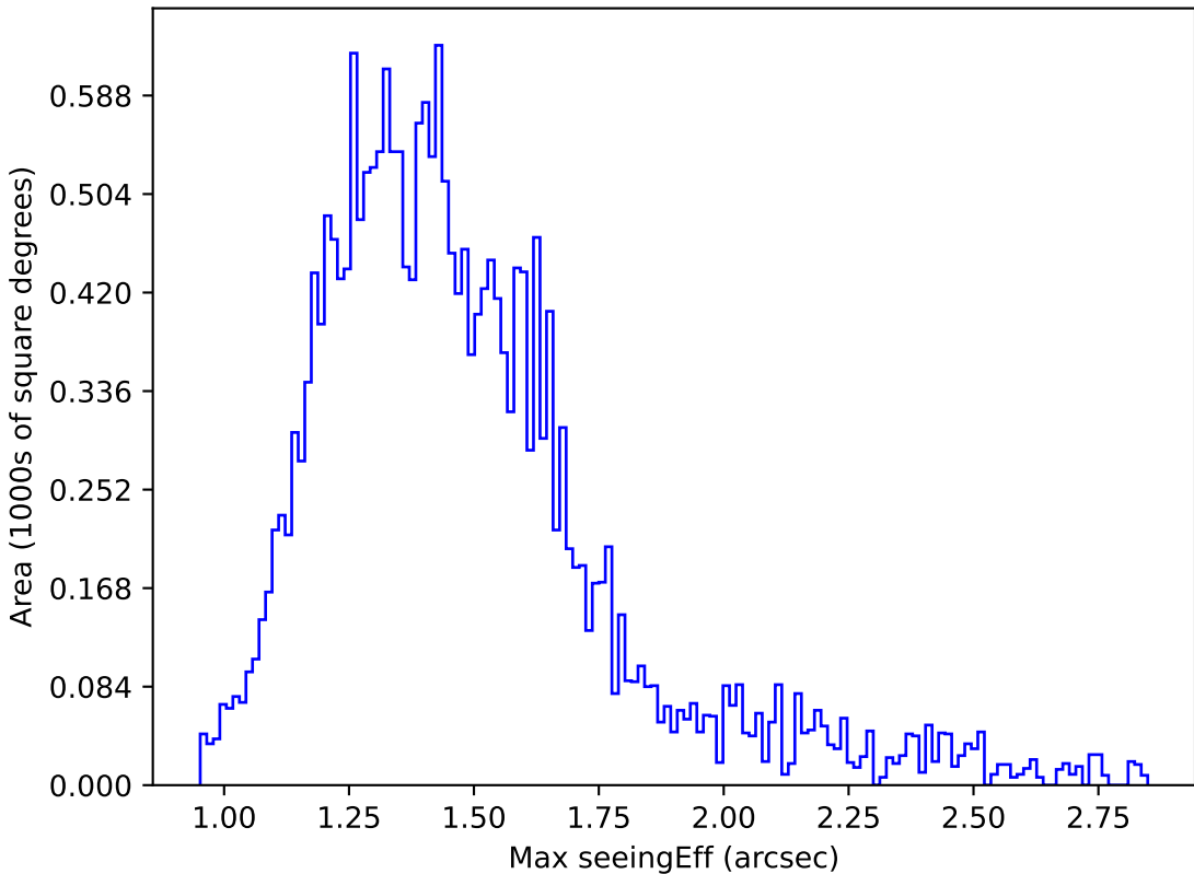
too_elab_heavy_r32_d3_gz_v3.4_10yrs Yr 1 y band: Max seeingEff
