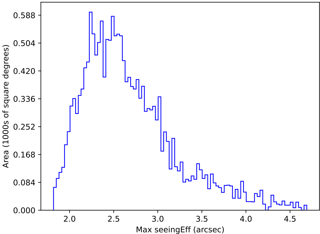
too_elab_heavy_r32_d3_gz_v3.4_10yrs WFD r band: Max seeingEff
