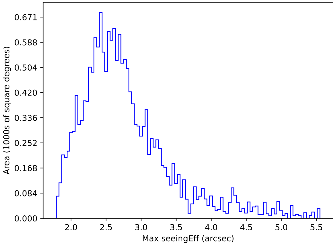
too_elab_heavy_r32_d3_gz_v3.4_10yrs WFD i band: Max seeingEff
