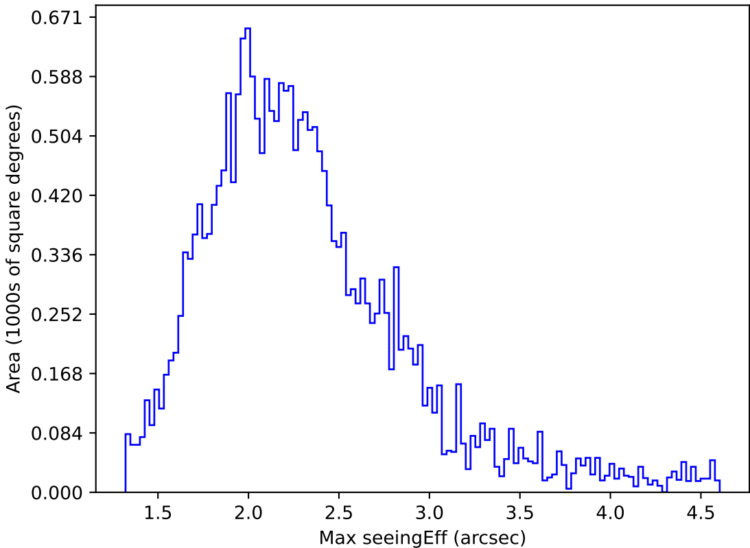
too_elab_heavy_r32_d3_gz_v3.4_10yrs All sky y band: Max seeingEff
