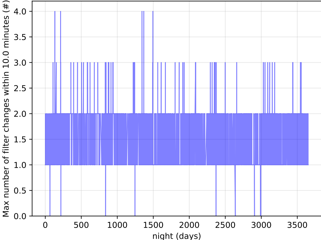
too_elab_heavy_r32_d3_gz_v3.4_10yrs Per Night: Max number of filter changes within 10.0 minutes
