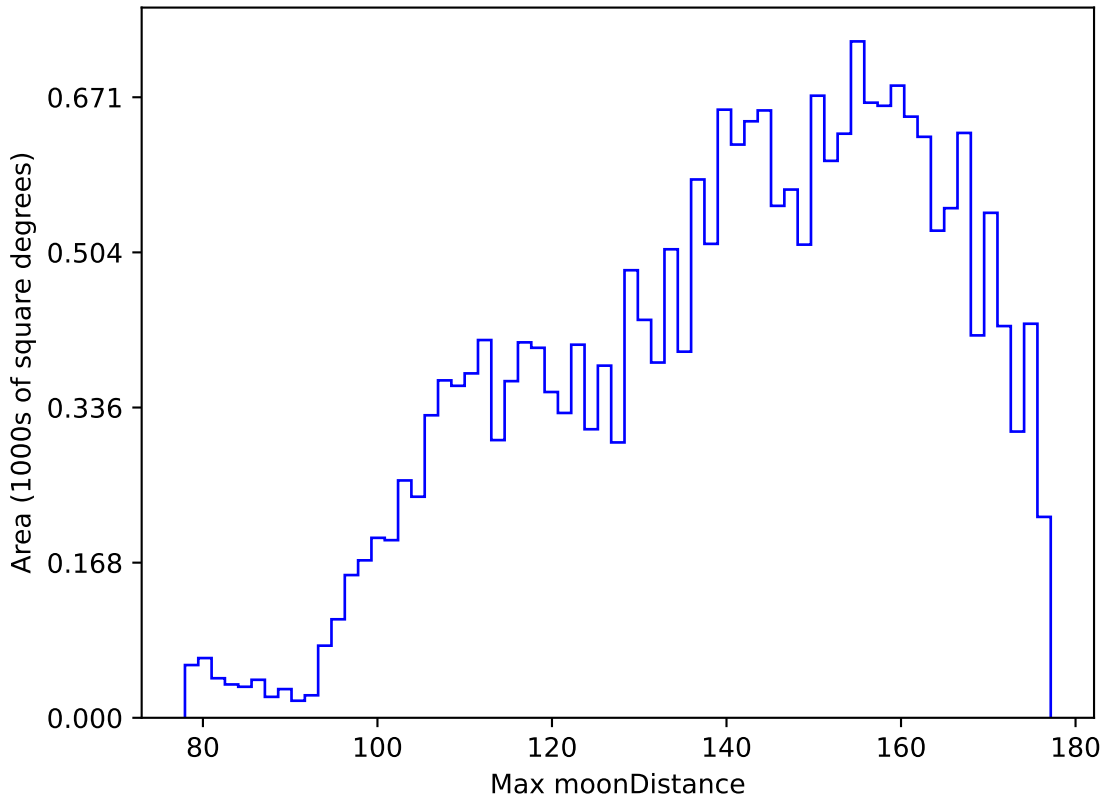
too_elab_heavy_r32_d3_gz_v3.4_10yrs All sky y band: Max moonDistance
