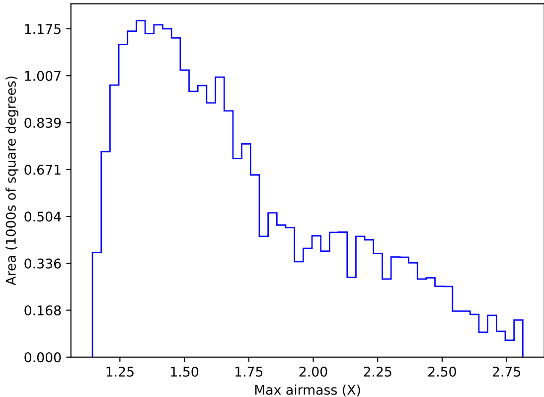
too_elab_heavy_r32_d3_gz_v3.4_10yrs Yr 1 z band: Max airmass
