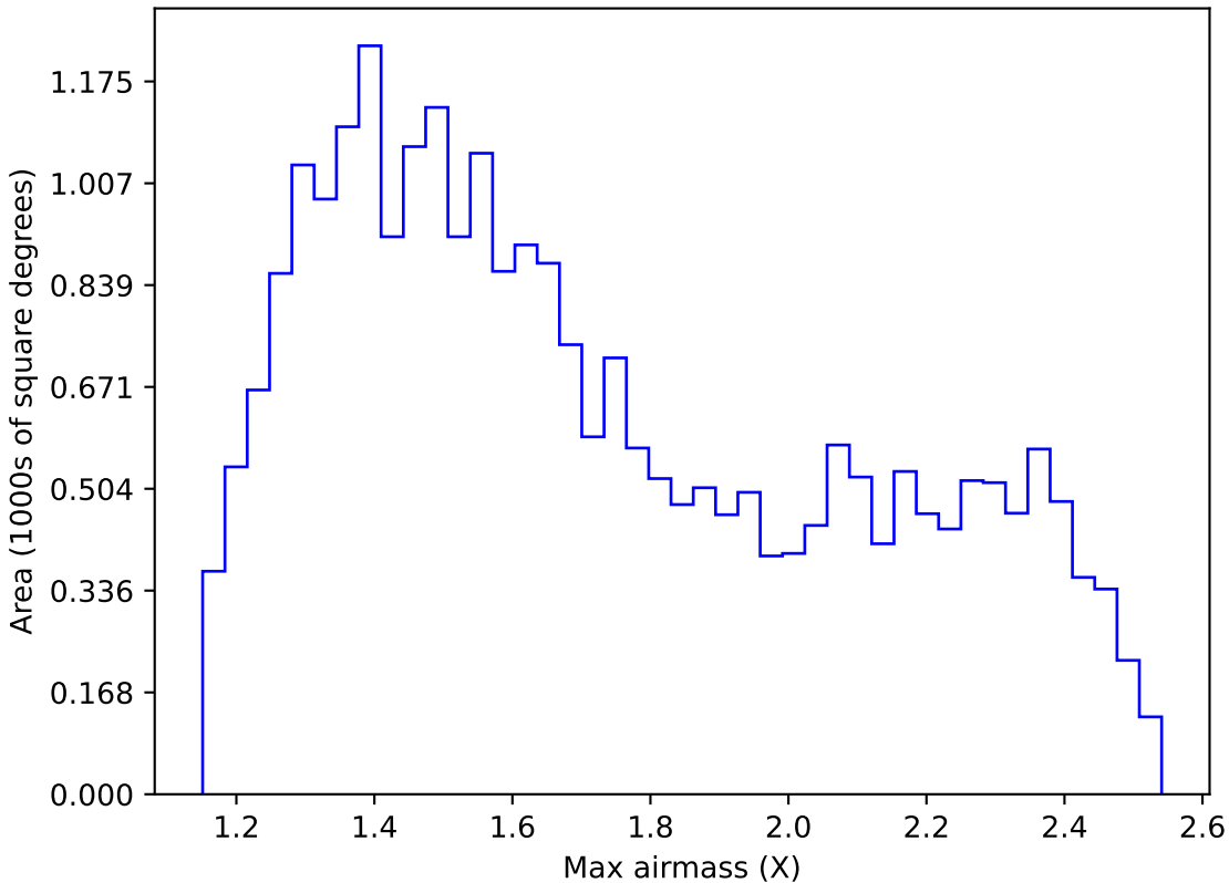
too_elab_heavy_r32_d3_gz_v3.4_10yrs Yr 1 r band: Max airmass
