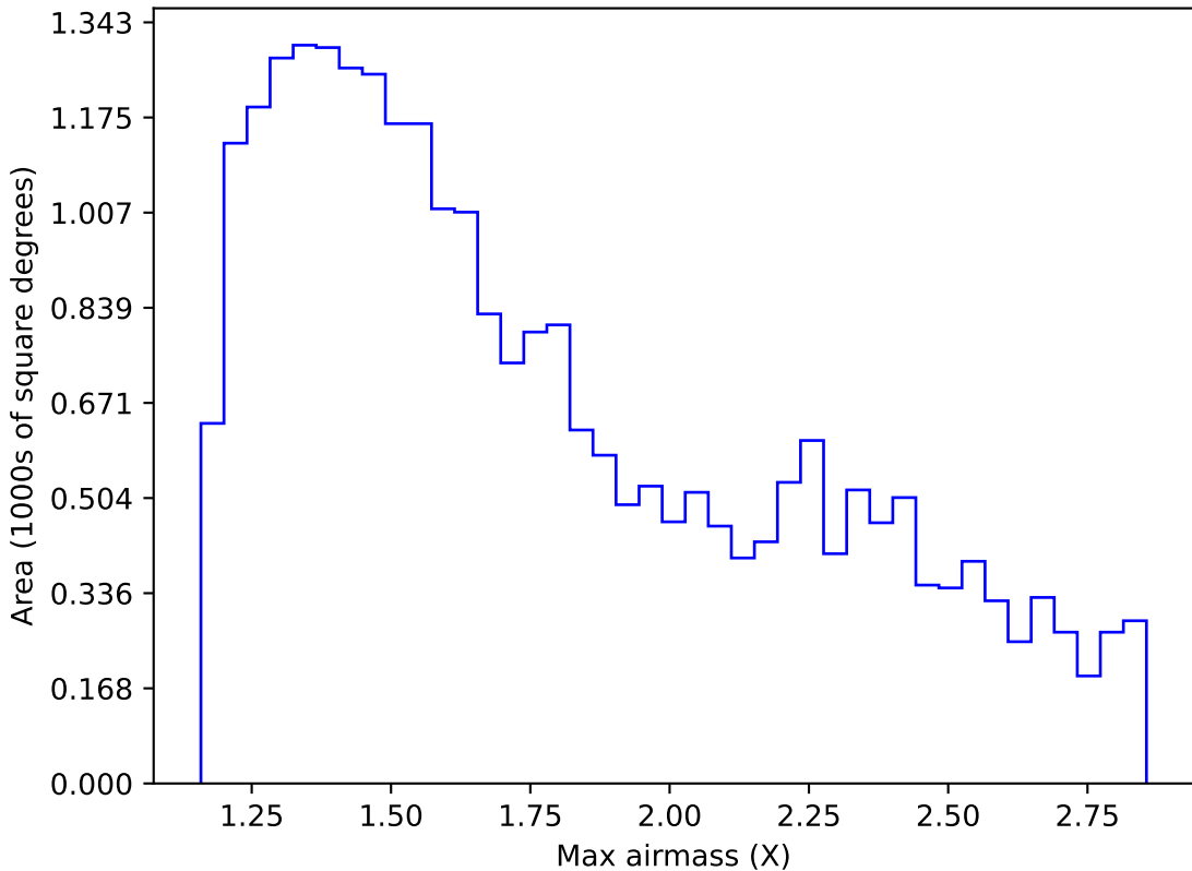
too_elab_heavy_r32_d3_gz_v3.4_10yrs Yr 1 i band: Max airmass
