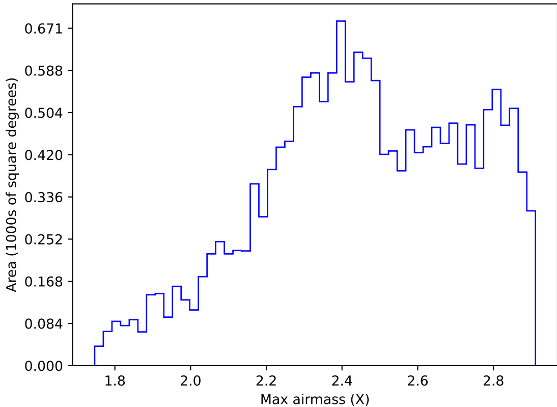
too_elab_heavy_r32_d3_gz_v3.4_10yrs WFD z band: Max airmass
