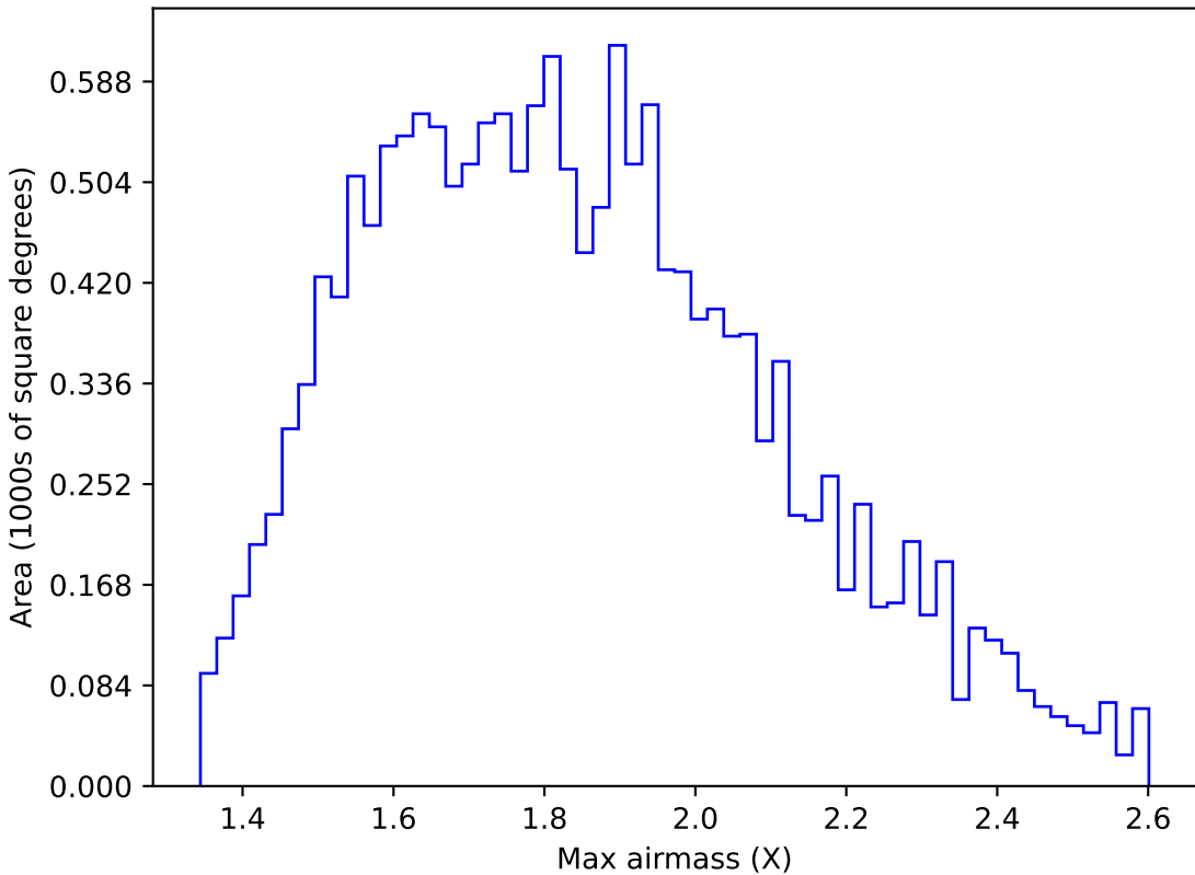
too_elab_heavy_r32_d3_gz_v3.4_10yrs WFD u band: Max airmass
