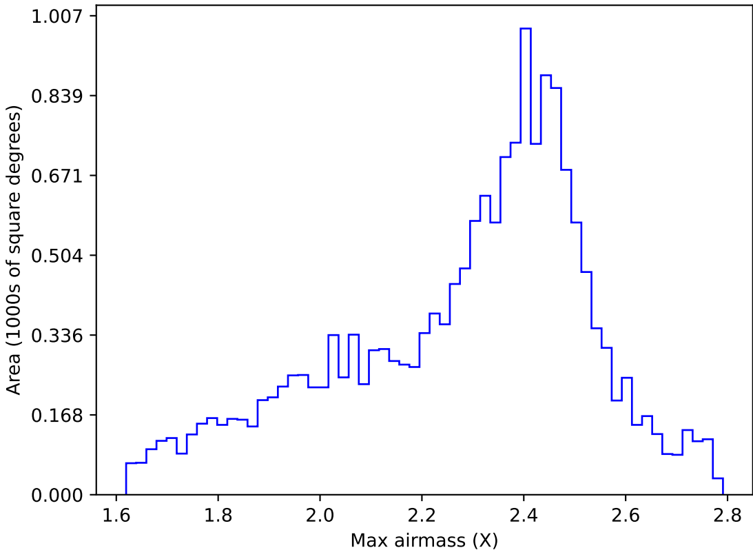
too_elab_heavy_r32_d3_gz_v3.4_10yrs WFD r band: Max airmass
