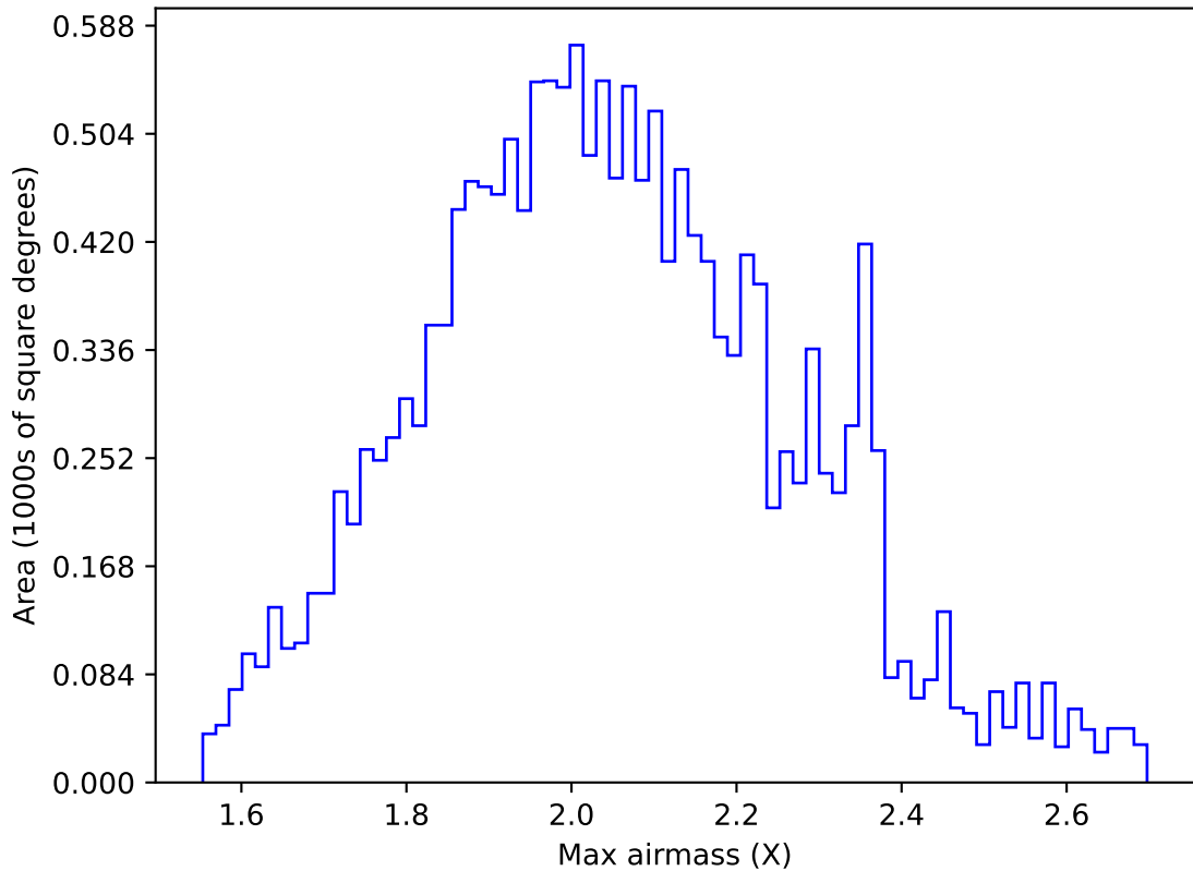
too_elab_heavy_r32_d3_gz_v3.4_10yrs WFD g band: Max airmass
