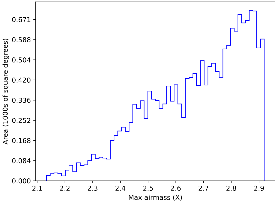
too_elab_heavy_r32_d3_gz_v3.4_10yrs WFD all bands: Max airmass
