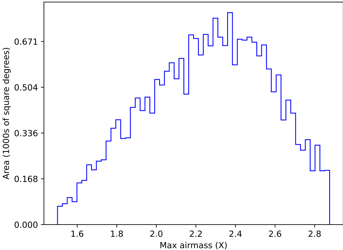
too_elab_heavy_r32_d3_gz_v3.4_10yrs All sky y band: Max airmass
