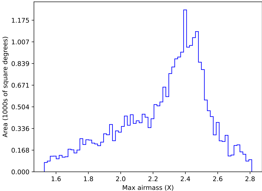
too_elab_heavy_r32_d3_gz_v3.4_10yrs All sky r band: Max airmass
